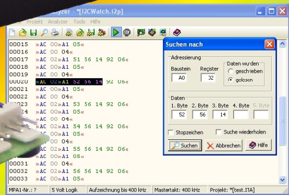
I 2 C-Analyzer/Monitor
